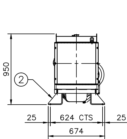
MUFFLER 2" PIPES
